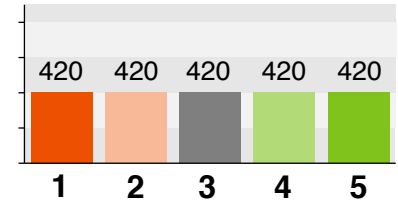
ArguAnaTripAdvisor corpus
